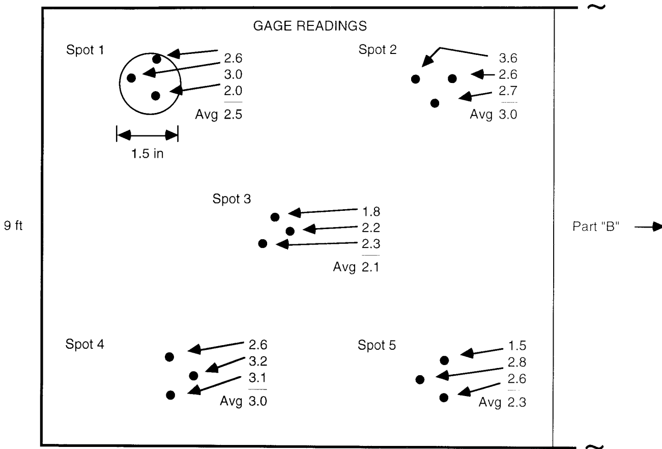
FIGURE A1 Part "A" of Structure (Area Approx. 10 m 2 [100 ft 2 ])
